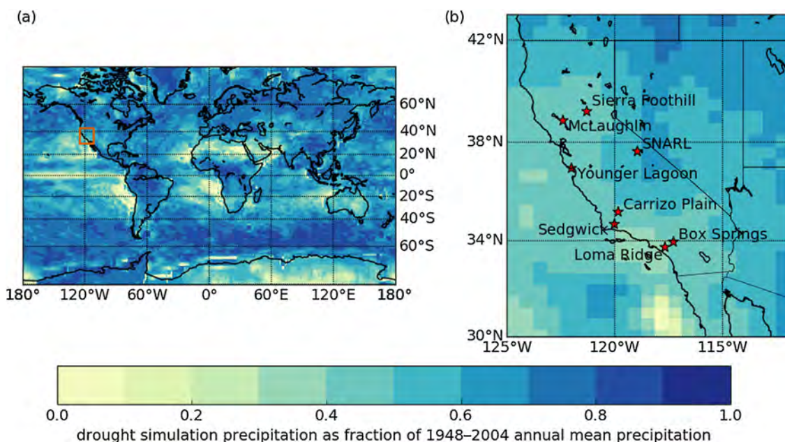
Fig. 1. International Drought Experiment (IDE) per-gridcell precipitation reduction. Panel (a): global precipitation reduction as a fraction of the 1948–2004 annual mean total precipitation. Panel (b): as panel (a), but zoomed to the California, USA analysis area (shown in the orange box in panel (a)). Precipitation reduction fractions are calculated as ((1st percentile)/(50th percentile)) of the 1948–2004 (Qian et al., 2006) annual total precipitation (see Section 2). Red stars on the panel (b) denote the California analysis sites described in Table 1. (For interpretation of the references to color in this figure legend, the reader is referred to the web version of this article.)
